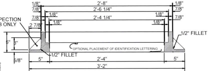
STORM SEWER INLET FRAME NEENAH R-3076 OR AN APPROVED EQUAL
