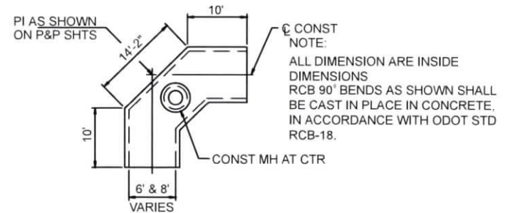
RCB 90° BEND DETAIL
