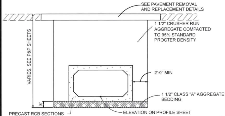
RCB DETAIL - PAVED AREAS
