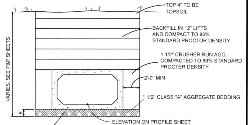
RCB DETAIL - OPEN AREAS
