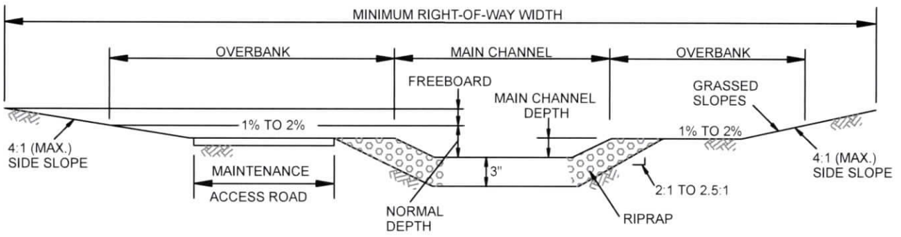
SECTION
