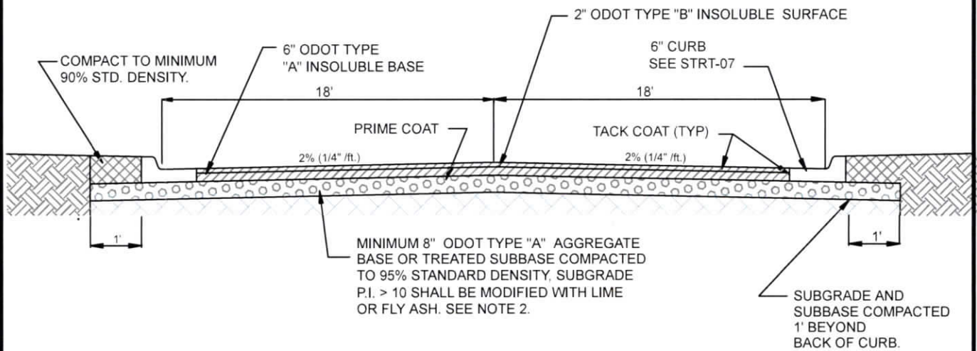
ASPHALTIC CONCRETE STREET SECTION
