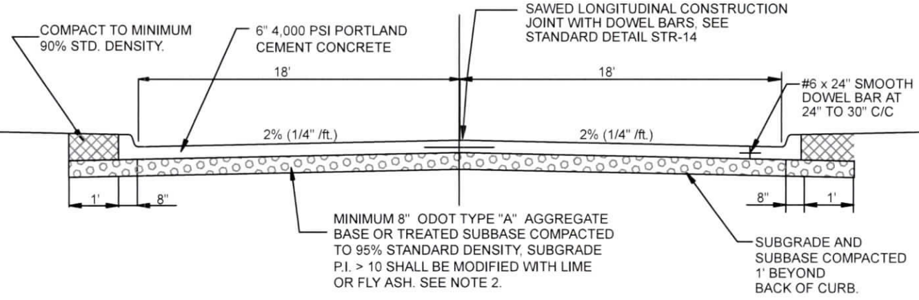
CONCRETE STREET SECTION
