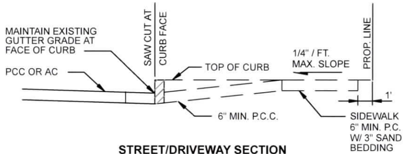
STREET/DRIVEWAY SECTION
