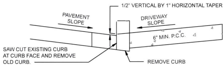
SECTION AT GUTTER
