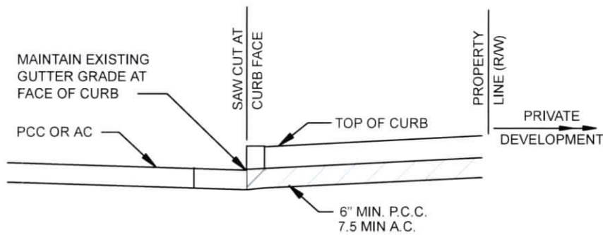
STREET/DRIVEWAY SECTION
