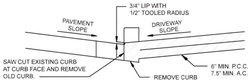
SECTION AT GUTTER
