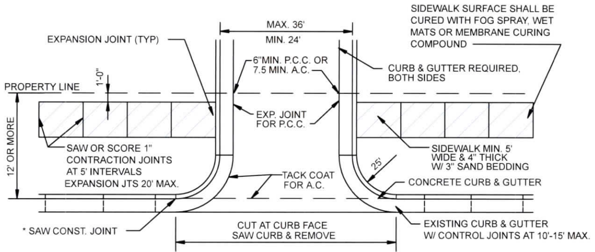
REGULAR DRIVE
