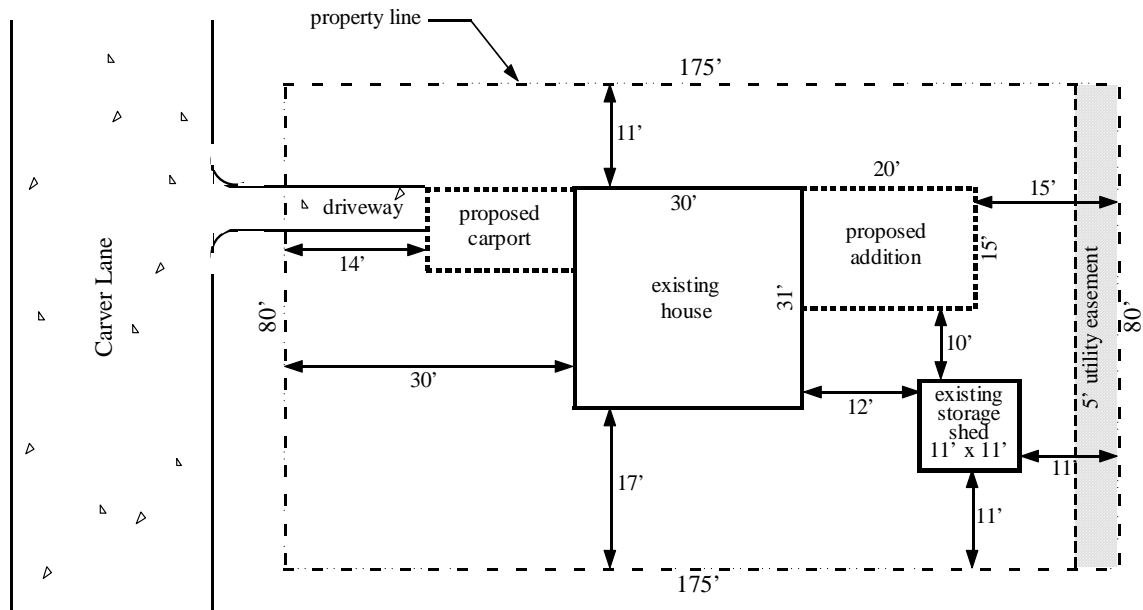
SAMPLE SITE PLAN
